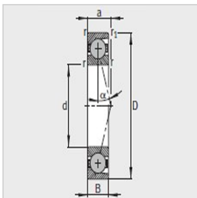
HCB719...-C、HCB70...-C、HCB72...-C \alpha = 15^\circ
