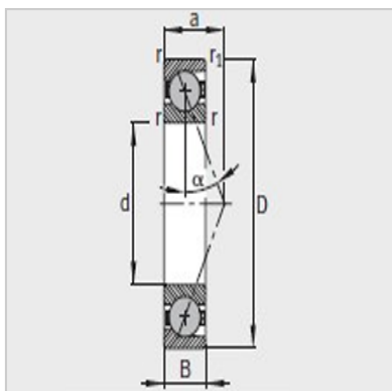
HCB719...-E、HCB70...-E、HCB72...-E \alpha = 25^\circ
